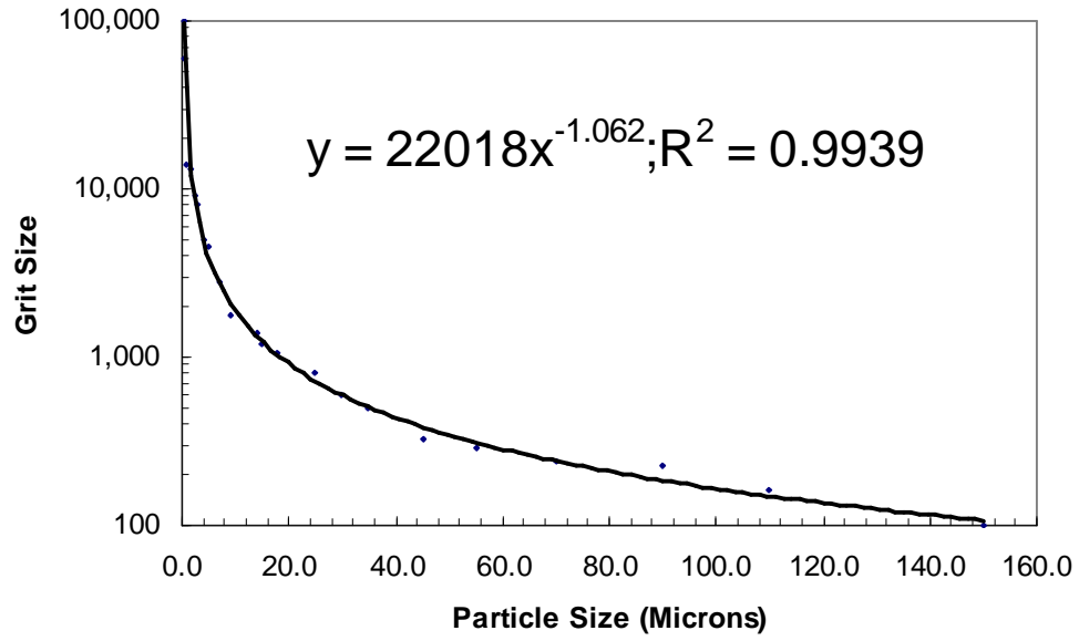
American Grit Size as a Function of Particle Size in Microns
